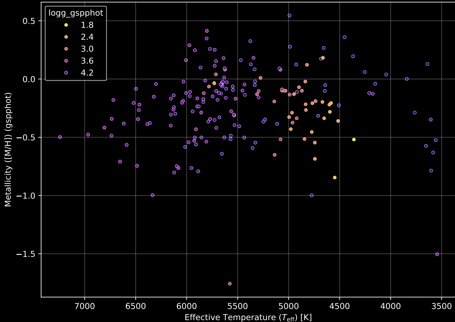
APOGEE DR17 Field: [189+47_MGA] Stellar Population Parameters (n= 189)
