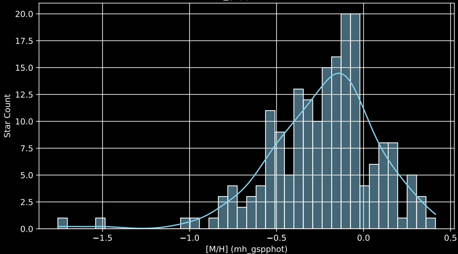
APOGEE DR17 Field: [189+47_MGA [M/H] (mh_gspphot) (n= 188)
