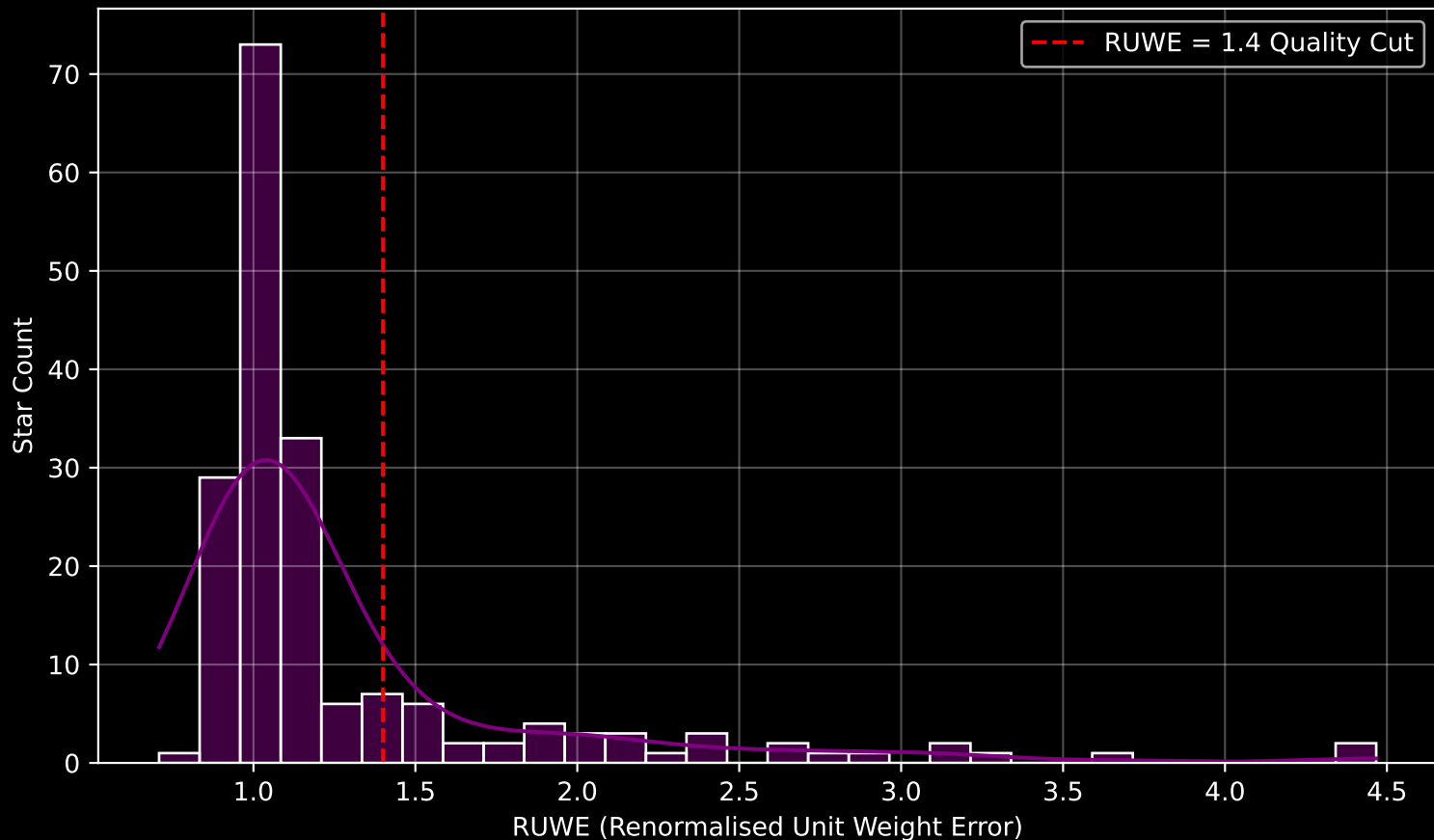
GAPOGEE DR17 Field [189+47_MGA] RUWE Distribution (n= 183)
