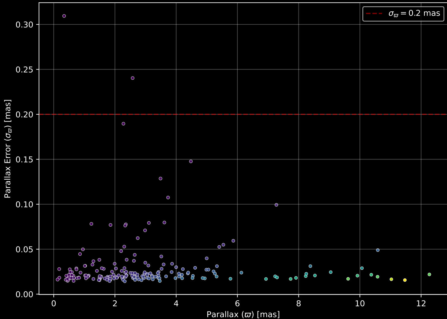
APOGEE DR17 Field: [189+47_MGA] Parallax Quality (n= 189)
