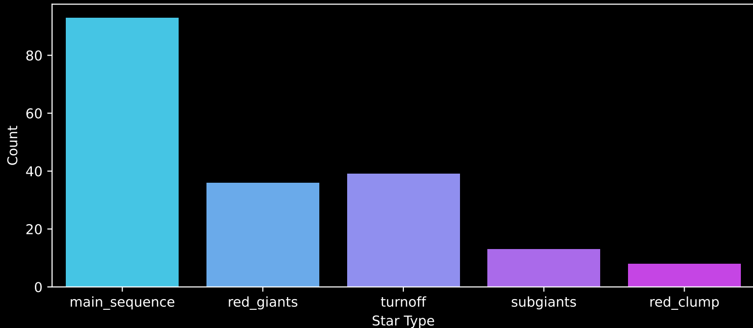
APOGEE DR17 Field: [189+47_MGA] Count plot of Star Type
