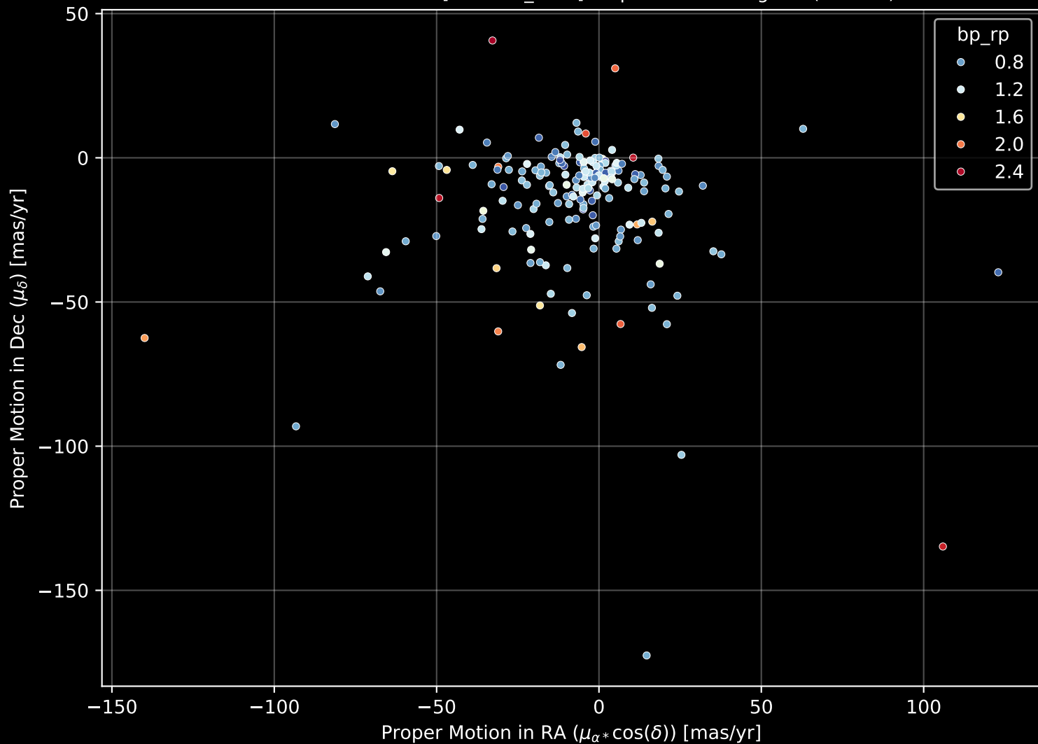
APOGEE DR17 Field: [189+47_MGA] Proper Motion Diagram (n= 189)
